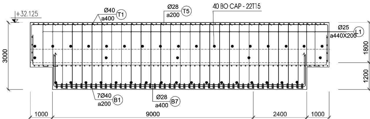
Fig. 7 Structure of reinforced beams.
