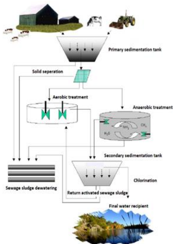
Fig. 1 Flowchart of Livestock WWTP [8].
